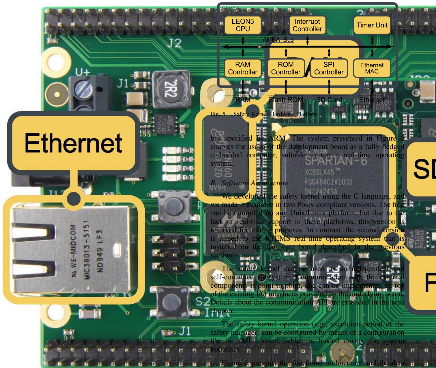
Fig. 4. Safety Kernel Hardware Platform
