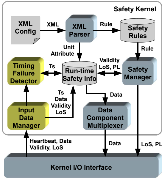
Fig. 6. Functional architecture
